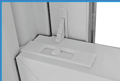
Vent Latch when deployed, will limit sash travel to allow for ventilation.
